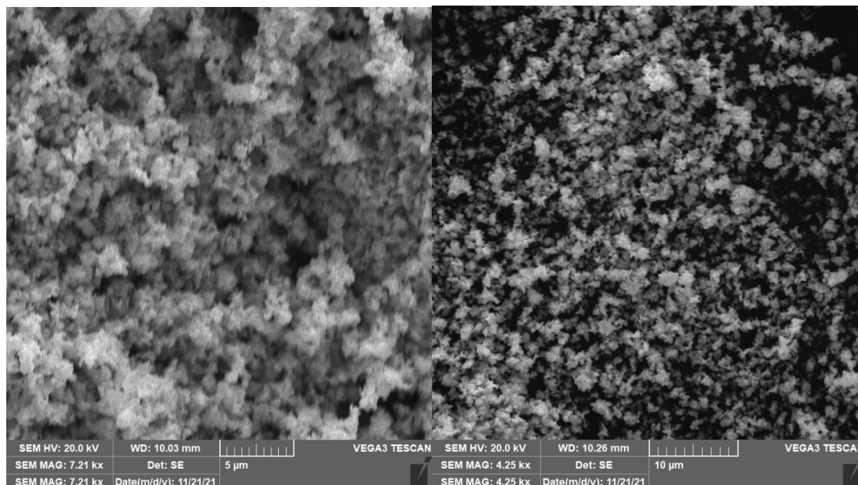
Figure 4. SEM images of zinc oxide nanoparticles with different magnifications (left 5 μm) and (right 10 μm).
